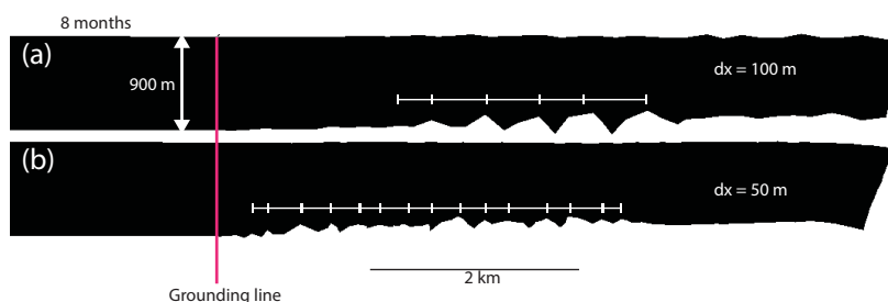
Figure 8. Geometries of the mesh for a resolution of (a) 100 m and (b) 50 m. The pinch-and-swallow features (“boudins”) appear with regularity (white bars) and decreasing size upon mesh refinement. Computational limitations precluded running the simulations at quartered resolution.
