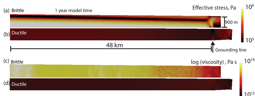
Figure 5. Effective stresses in (a) purely brittle and (b) purely ductile ice for wedge experiments after 1 year of model time. The left nodes vary freely in the vertical and are fixed to 0 in the horizontal, and the basal boundary is free-slip. There is an order-of-magnitude difference in stress. Again, brittle ice experiences a small process zone of high stress immediately at the grounding line (black arrow) where there is a transition from freely slipping ice to a buoyancy stress condition with a 1 m diurnal tidal forcing, and the forces due to bending are high. Ductile ice also experiences an increase in stress at this location, although the transition is not as sharp. Most notably, flow in brittle ice is negligible compared to ductile ice after 1 year, owing to the very large (as much as 5 orders of magnitude) difference in viscosity between the (c) brittle and (d) ductile ice.
