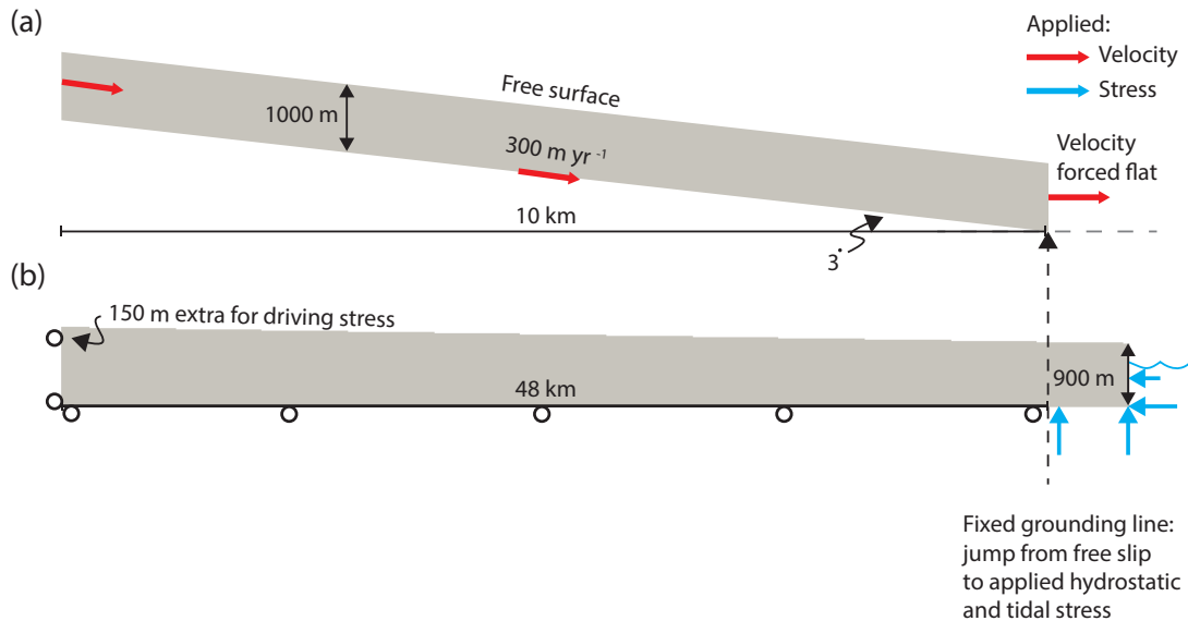
Figure 2. Schematic of experiments. (a) Experiments performed with a purely ductile or brittle rheology are initialized as a parallel-sided slab that is advected down a plane and forced flat at 10 km. (b) Setup for semi-brittle rheology: a horizontal domain of 50 km and a fixed grounding line at 48 km, with an initial 2 km of floating tongue. The left-hand side horizontal velocity is fixed at 0, and the bottom side upstream (left) of the grounding line vertical velocity is fixed at 0 (this type of boundary condition is represented schematically by open black circles). Hydrostatic and tidal stress is applied to the bottom and right-hand side of the domain downstream (right) of the grounding line.
