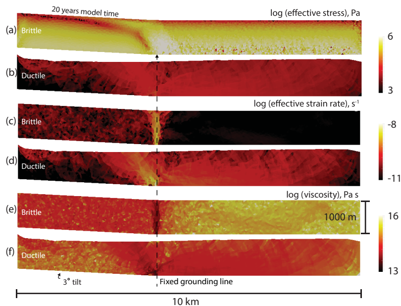
Figure 3. Comparisons of purely brittle (a, c, e) and purely ductile (b, d, f) tilted-slab experiments. (a, b) Effective stress, (c, d) effective strain rate, and (e, f) viscosity after 20 years of model time. Overall the brittle rheology results in a narrow process zone of high stress and deformation, while the ductile rheology has a more diffuse area of strain and lower stresses.
