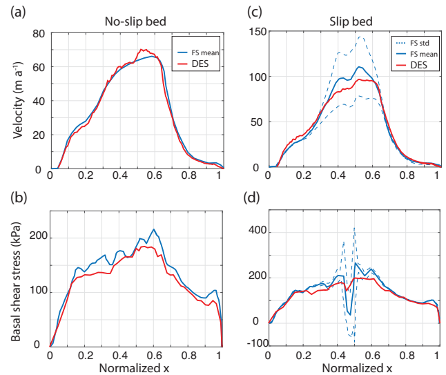
Figure B1. DES with semi-brittle ice executed according to experiment E presented by Pattyn et al. (2008). (a) Surface velocity and (b) basal shear stress for ice completely frozen to the bed, and (c) surface velocity and (d) basal shear stress for ice with a freely slipping patch for a small portion of the domain. Full Stokes (FS, blue line) model means compare reasonably with those from DES (red line).
