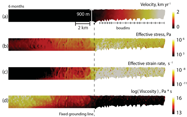
Figure 6. Simulation of semi-brittle wedge of ice after 6 months of model time, undergoing a jump in boundary conditions from freely slipping on the basal side (left of grounding line – dashed arrow) to floating in the ocean (right of grounding line). The horizontal velocity ( a ) is fixed at x = 0 and free elsewhere, while the vertical velocity is free at x = 0 and fixed to 0 up to the grounding line. The gradient in thickness drives the flow of ice over the grounding line where ice experiences a transition to stress boundary conditions that represent floatation and 1 m tides. Dashed bars in the floating tongue show the development of boudins. The effective stress ( b ) and strain rate ( c ) fields both show orders-of-magnitude increases at the grounding line: the jump in strain rate allows the ice to be evaluated as brittle in DES, and the associated stresses are high enough to reach yield (see Fig. 6). The corresponding viscosities ( d ) just upstream of the grounding line are high and decrease 3 orders of magnitude as the ice expands out into the ocean under its own weight.
