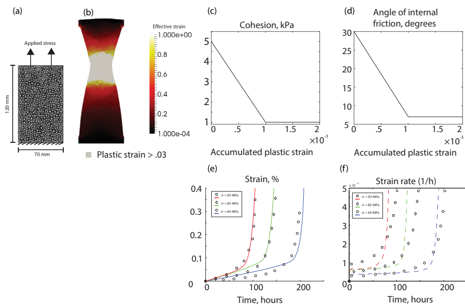
Figure A1. Calibration experiments for semi-brittle ice based on laboratory-derived data presented in Mahrenholtz and Wu (1992). (a) Initial mesh and dimensions and (b) effective strain after failure of semi-brittle ice with 0.82 MPa applied vertical stress. Overlaid on top is the accumulated plastic strain (grey) of elements > 0.03 . Because the grey extends horizontally throughout the ice plug, we consider an accumulated plastic strain of 0.03 or greater to represent ruptured ice. (c) Cohesion and (d) angle of internal friction parameters that are needed as a function of accumulated plastic strain to reproduce the (e) strain- and (f) strain-rate-vs.-time curves presented in Mahrenholtz and Wu (1992). Open black points are laboratory-derived data, and colored lines are from DES experiments.
