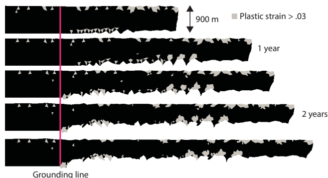
Figure 7. Plastic strain over 2.5 years of model time. Ice fails in tension at the surface near the terminus with regularity at the grounding line where hydrostatic stress is applied (in pink). Ice forms boudin-like features after accommodating a large amount of strain.
